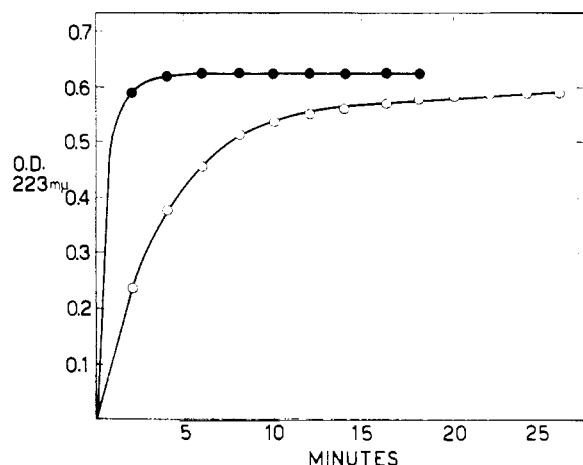
FIG. 1.—Oxidation of 2,5-diketohehexose with sodium periodate before and after reduction with \text{NaBH}_4 . Filled circles: 2,5-diketohehexose. Open circles: mixture of the three hexitols derived from 2,5-diketohehexose reduction. The enzymic product prepared as described in Table I was purified by ion-exchange chromatography and bromine oxidation as described under "Identification of 2,5-diketohehexose." The two curves were obtained with amounts of the product equivalent to 1/1000 of the original incubation mixture (Table I). One aliquot was reduced with \text{NaBH}_4 and treated as described in the text; the other had received no further treatment before reaction with periodate. An increase in optical density of 0.5 corresponds to the complete oxidation of 0.01 \mu\text{moles} of a mannitol standard.
